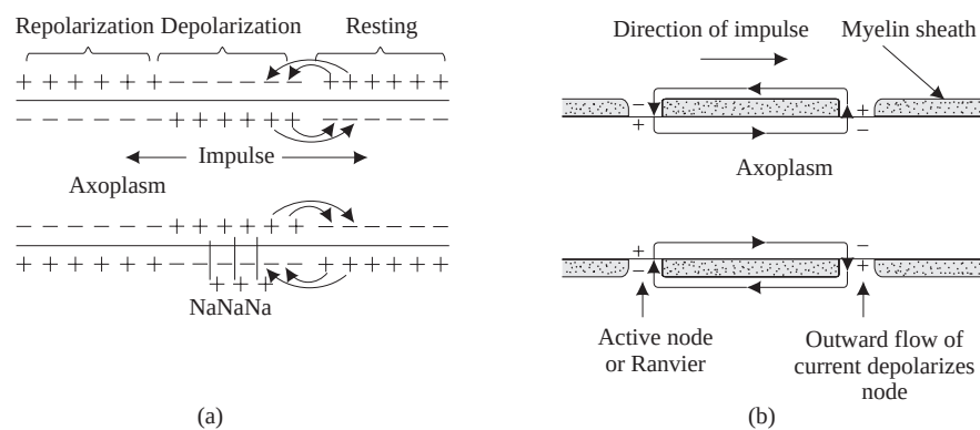
Fig. 15.13 Diagram illustrating the local circuit theory in (a) nonmyelinated fibre and (b) myelinated fibre (saltatory conduction). (After A.L. Hodgkin (1957), Proc. Roy. Soc. B. 148)
