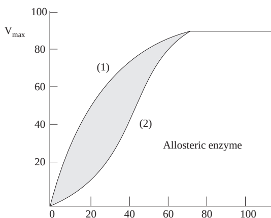
Fig. 4.11 Effect so substrate concentration on the velocity of (1) an enzyme showing Michaelis-Menten kinetics and, (2) allosteric enzyme.
