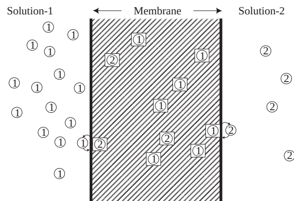
Fig 8.2 Exchange diffusion: The carrier in the membrane forms complexes with the ions. When the carrier with the ion of solution-1 reaches the membrane surface facing the solution-2, a 1:1 exchange of ions takes place between the carrier-ion complex of that solution. Similar 1:1 exchange of ions would take place if the carrier carrying ion of solution-2 reaches the membrane surface facing solution-1.
